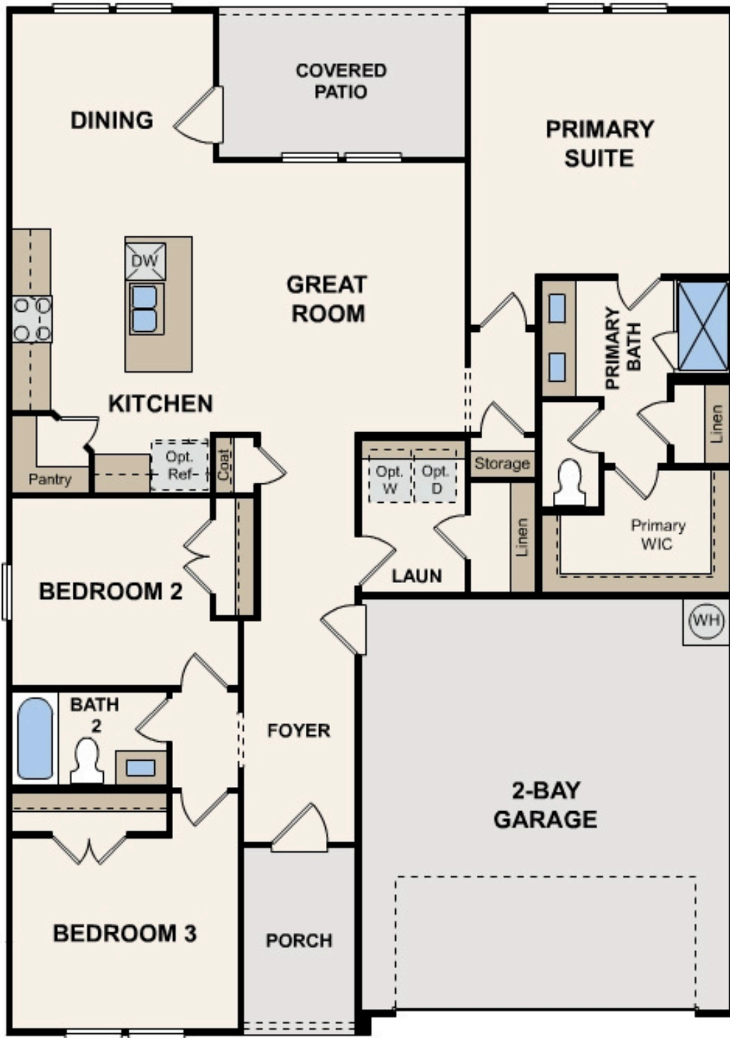
FLOOR PLAN
